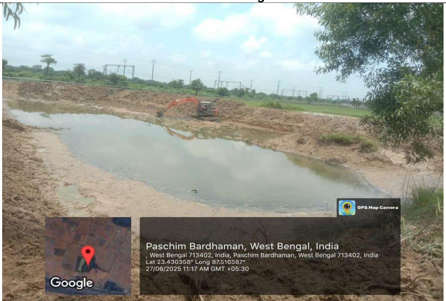
Storage Pond for Ground Water Recharge through Rain Water Harvesting
